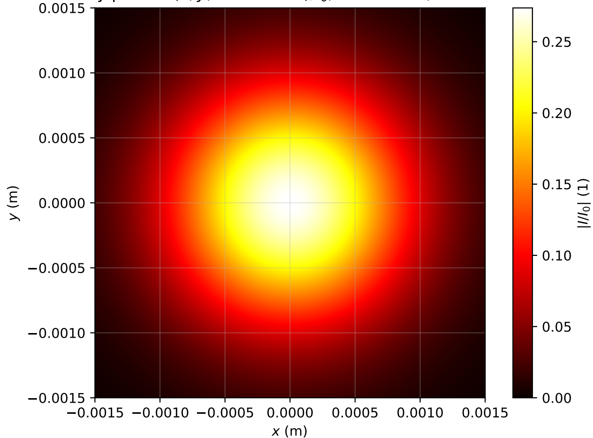
Intensity profile I(x, y, z = 3.742m)/I_0 , P_{in}=0.2P_{cr} , artificial time
